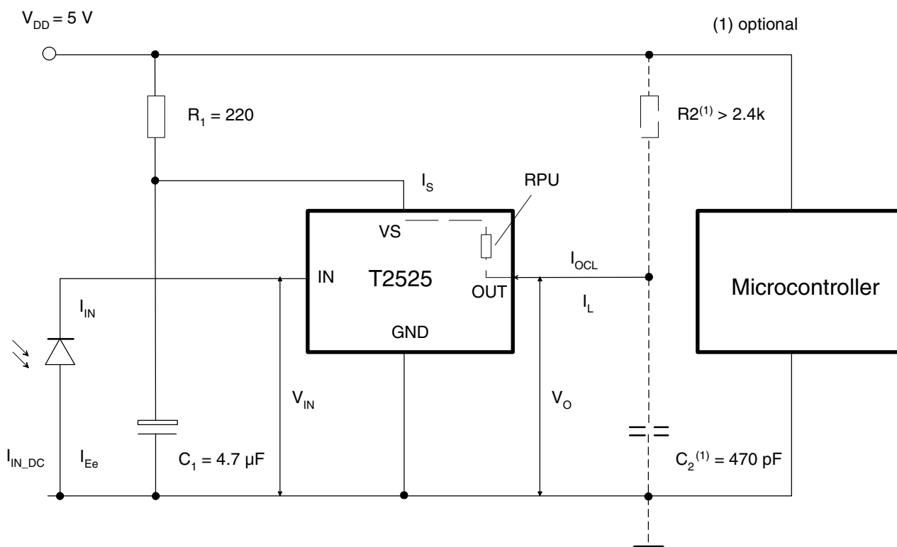
Figure 9. Application Circuit
