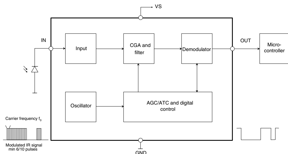
Figure 1. Block Diagram
